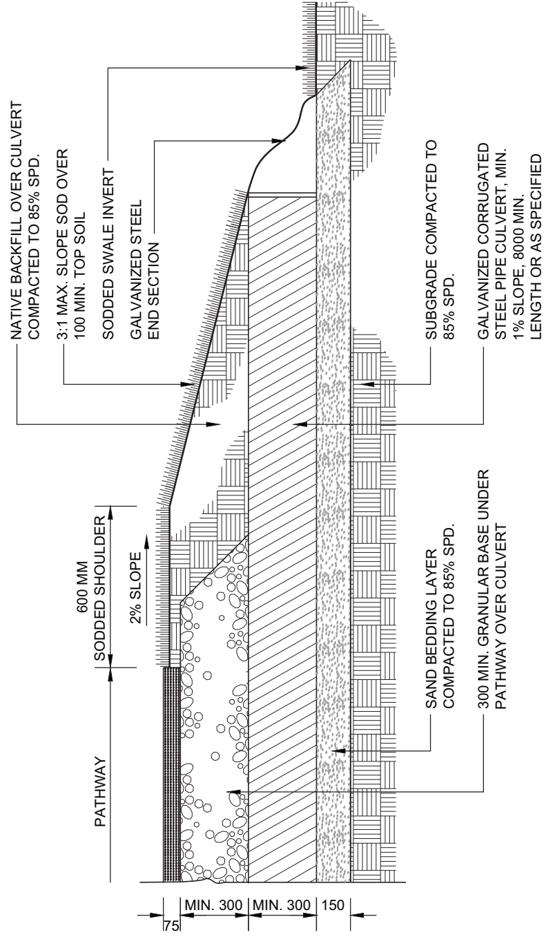
SECTION
